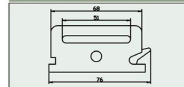
2" End Fitting F010301
