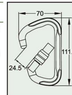
D1 Carabiner C3101 series Forged Aluminum Alloy Screw Lock Snag-free Design Anodized Min. Breaking Strength: 23kN/5000lbs
