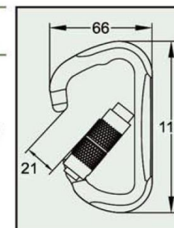
D1 Carabiner C3102 series Forged Aluminum Alloy Twist Lock Snag-free Design Anodized Min. Breaking Strength: 23kN/5000lbs
