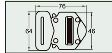
Harness Safety Buckle K0601 series
