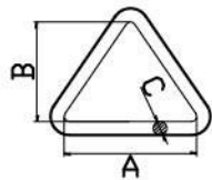
Triangle Ring RING-05
