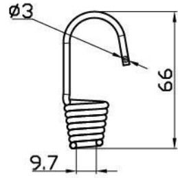
Bungee Hook-01 SPR02 SUS304
