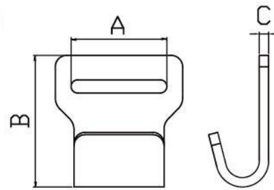
Flat hook-02 FTH-002
