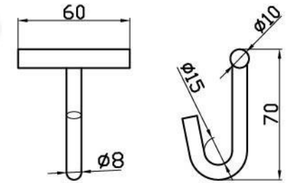
Welding Tube Single Hook J-Hook-07
