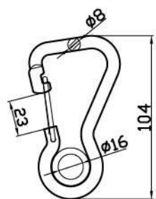
Spring Hook SPRING HOOK-02
