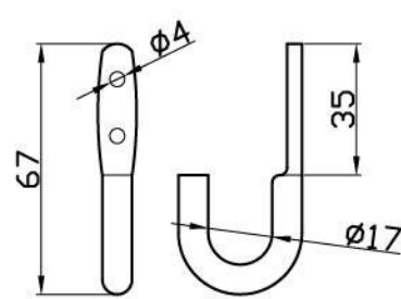
J Shaped Tie Hook J16-060060Z
