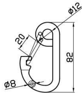
Spring Hook WH08P
