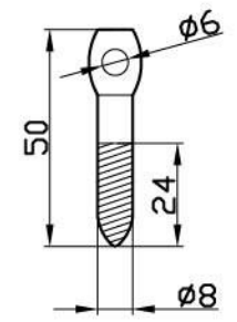
Bolt/Eyelet Screw Bolt-02
