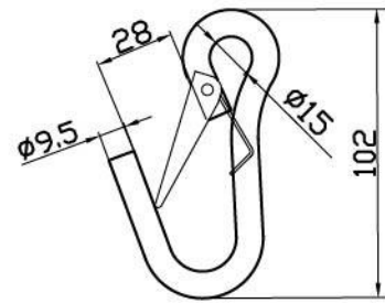
Snap Hook SH04P
