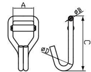
Eye Hook J-Hook-09
