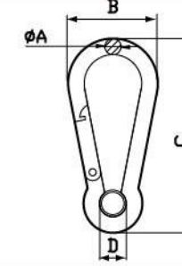
Snap Hook with Eyelet SNAP HOOK-01
