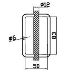
Buckle with Anti-slip Adjuster Buckle-02
