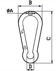
Snap Hook SNAP HOOK-02
