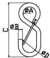
S Hook with Spring S HOOK-04
