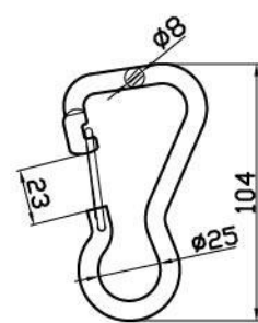
Spring Hook SPRING HOOK-01
