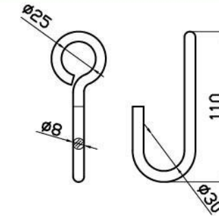
Finger Profile Hook J-Hook-06
