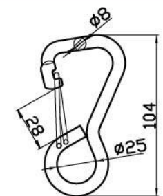
Spring Hook SPRING HOOK-03
