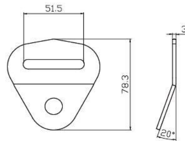
2" Delta Flat Hook FTH-004
