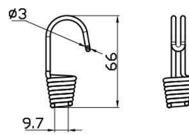
Bungee Hook-02 SPR03 SUS304
