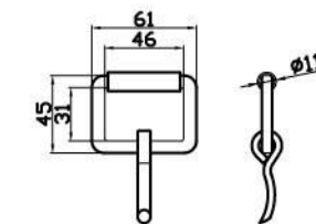
Tongue Buckle Buckle-04
