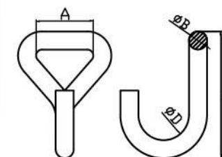
J Hook J-Hook-10
