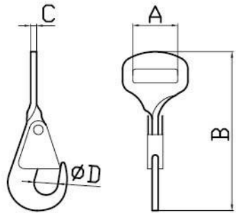
Twist Snap Hook FTH-003
