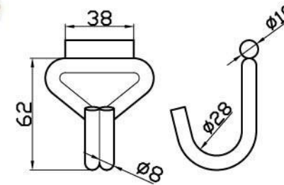
Welding Tube Profile Hook J-Hook-08
