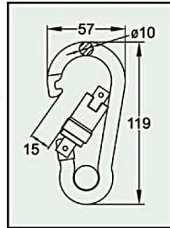
WAIST Carabiner C4203 series Alloy Steel One-way Lock Min. Breaking Strength: 23kN/5000lbs
