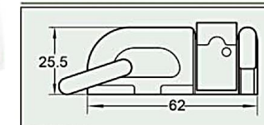
Double Stud Fitting with O ring M071138
