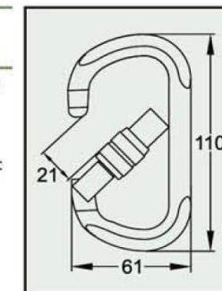
D Carabiner C2101 series Forged Aluminum Alloy Screw Lock Snag-free Design Anodized Min. Breaking Strength: 23kN/5000lbs
