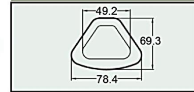
Buckle-05 F44 series
