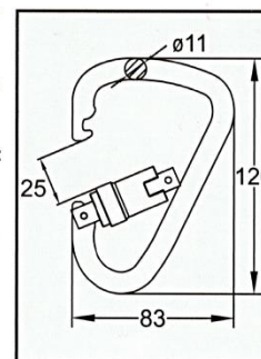
D1 Carabiner C3203 series Alloy Steel One-way Lock Min. Breaking Strength: 23kN/5000lbs
