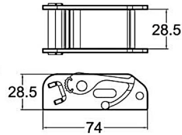
1" Steel Cam Buckle K010104~08 Size: 1"/25mm B.S: 500kg Finish: Electric black plated Optional Color Button Scratch proof pad
