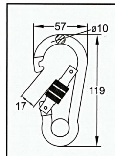
WAIST Carabiner C4201 series Alloy Steel Screw Lock Min. Breaking Strength: 23kN/5000lbs
