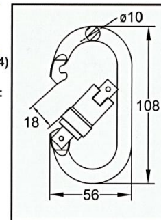
C Carabiner C1303 series Stainless Steel(SUS 304) One-way Lock Min. Breaking Strength: 10kN/2500lbs
