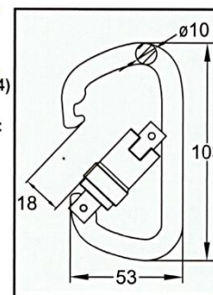
D Carabiner C2303 series Stainless Steel(SUS 304) One-way Lock Min. Breaking Strength: 10kN/2500lbs
