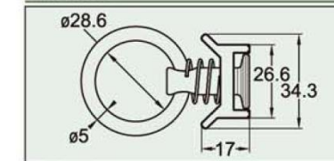
Single Stud Fitting M071105
