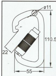
D1 Carabiner C3202 series Alloy Steel Twist Lock Min. Breaking Strength: 23kN/5000lbs
