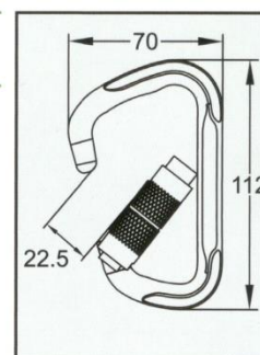
D1 Carabiner CBRAD1-F-002 Forged Alloy Steel Twist Steel Lock Snag-Free Design Min. Breaking Strength: 40kN/8900lbs ANSI Certificated
