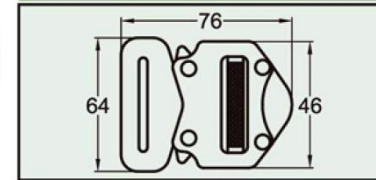
Harness Safety Buckle K0601 series
