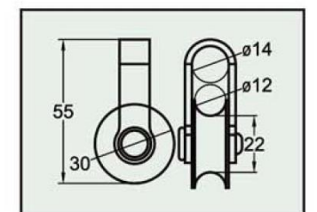
Pulley I0201 series Aluminum Alloy Anodized Webbing width : 12mm Min. Breaking Strength: 600kg/1300lbs
