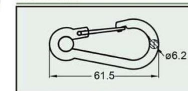
Wire Hook With Eyelet / Without Eyelet K08 Series
