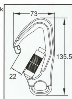
Twist Locking Snap Hook RBH-AL-M-001 Forged Aluminum Alloy Twist Lock Snag-free Design Anodized Min. Breaking Strength: 23kN/5000lbs EN362 Certificated
