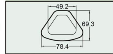
Buckle-05 F44 series
