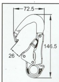
Self Locking Snap Hook RBH-M-AL-003 Forged Aluminum Alloy Anodized Min. Breaking Strength: 35kN/7500lbs EN362 Certificated
