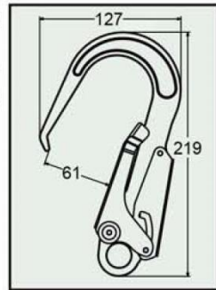
Self Locking Rebar Hook A0102 series Alloy Steel Min. Breaking Strength: 23kN/5000lbs
