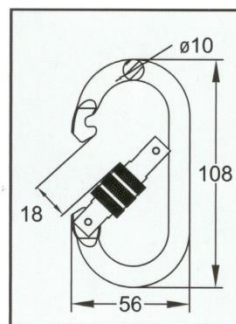
C Carabiner CBR-S-001 Alloy Steel Screw Lock Min. Breaking Strength: 23kN/5000lbs EN362 Certificated
