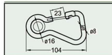
Spring Hook With Eyelet / Without Eyelet S02 Series
