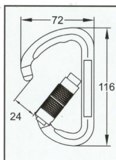
D1 Carabiner CBRAD1-ALF-004 Forged Aluminum Alloy Twist Lock Snag-free Design Anodized Min. Breaking Strength: 23kN/5000lbs EN362 Certificated
