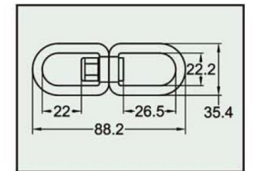
Swivel Connector - Medium I0202 series Forged Alloy Steel Yellow Zinc Plated / Chrome Plated Min. Breaking Strength: 23kN/5000lbs
