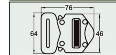
Harness Safety Buckle K0602 series
