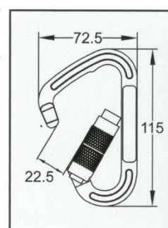
D1 Carabiner CBRAD1-ALF-001 Forged Aluminum Alloy Twist Lock Snag-Free Design Anodized Min. Breaking Strength: 23kN/5000lbs EN362 Certificated
