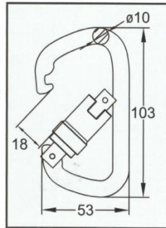
D Carabiner C2203 series Alloy Steel One-way Lock Min. Breaking Strength: 23kN/5000lbs
