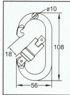
C Carabiner C1203 series Alloy Steel One-way Lock Min. Breaking Strength: 23kN/5000lbs
