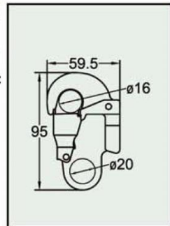
Self Locking Snap Hook A0302 series Alloy Steel Min. Breaking Strength: 23kN/5000lbs
