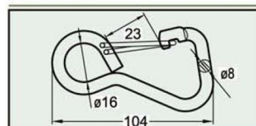
Spring Hook S02 Series
