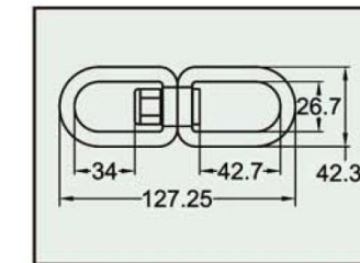
Swivel Connector - Large I0201 series Forged Alloy Steel Yellow Zinc Plated / Chrome Plated Min. Breaking Strength: 40kN/8900lbs
