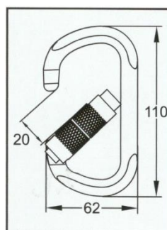
D Carabiner CBRAD-ALF-002 Forged Aluminum Alloy Twist Lock Snag-free Design Anodized Min. Breaking Strength: 23kN/5000lbs EN362 Certificated
