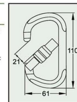
D Carabiner C2101 series Forged Aluminum Alloy Screw Lock Snag-free Design Anodized Min. Breaking Strength: 23kN/5000lbs
