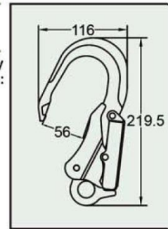
Aluminum Rebar Hook A0101 series Forged Aluminum Alloy Min. Breaking Strength: 23kN/5000lbs
