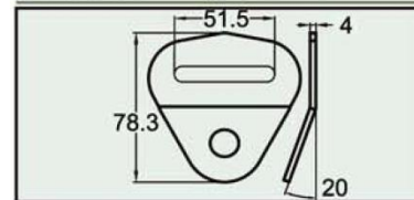
Delta Flat Hook F44 series
