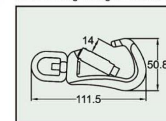
Swivel Connector I0201 series Forged Aluminum Alloy Twist Lock Snag-free Design Anodized Min. Breaking Strength: 9kN/2000lbs
