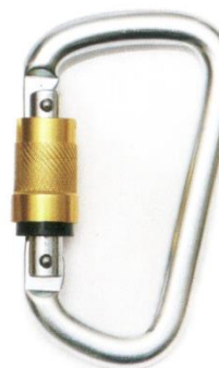
D Carabiner C2303 series Stainless Steel(SUS 304) One-way Lock Min. Breaking Strength: 10kN/2500lbs
