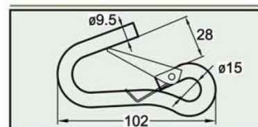
Snap Hook S11 Series
