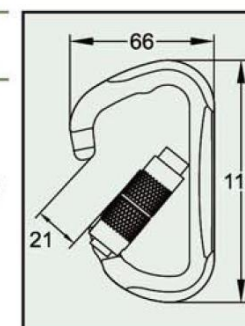
D1 Carabiner C3102 series Forged Aluminum Alloy Twist Lock Snag-free Design Anodized Min. Breaking Strength: 23kN/5000lbs
