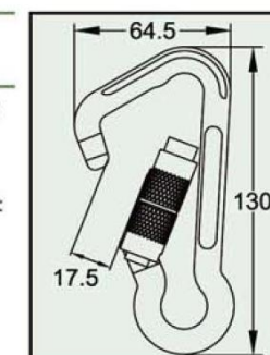
WAIST Carabiner C4102 series Forged Aluminum Alloy Twist Lock Snag-free Design Anodized Min. Breaking Strength: 23kN/5000lbs
