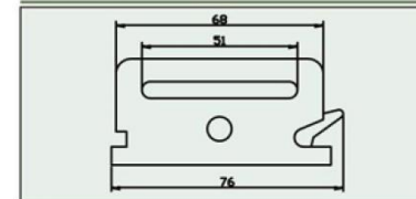
2" End Fitting F010301
