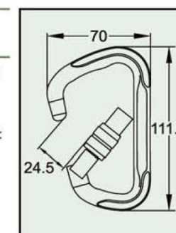
D1 Carabiner C3101 series Forged Aluminum Alloy Screw Lock Snag-free Design Anodized Min. Breaking Strength: 23kN/5000lbs
