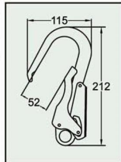
Self Locking Rebar Hook A0102 series Forged Alloy Steel Min. Breaking Strength: 23kN/5000lbs
