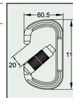
D Carabiner C2102 series Forged Aluminum Alloy Twist Lock Snag-free Design Anodized Min. Breaking Strength: 23kN/5000lbs
