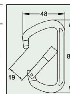
Quick Connector C2103 series Aluminum Alloy Quick Lock Snag-free Design Anodized Min. Breaking Strength: 9kN/2000lbs
