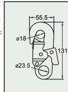
Self Locking Snap Hook A0202 series Alloy Steel Min. Breaking Strength: 23kN/5000lbs
