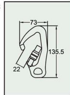
Screw Locking Snap Hook C5101 series Forged Aluminum Alloy Screw Lock Snag-free Design Anodized Titanium Min. Breaking Strength: 23kN/5000lbs
