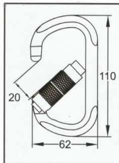
D Carabiner C2202 series Forged Alloy Steel Twist Lock Min. Breaking Strength: 23kN/5000lbs
